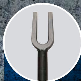
35939-02: T39B-2 BALL JOINT FORK FORK OPENING: 15/16" (2 CM)
